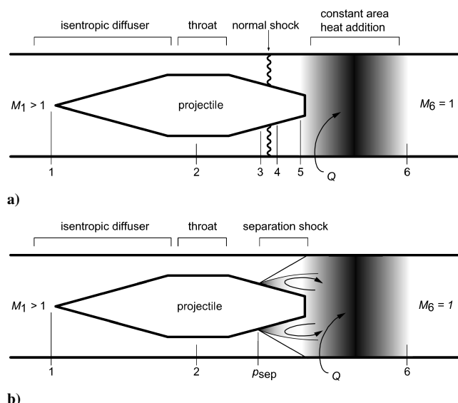
Fig. 5 Models of operation in thermally choked mode: a) one-dimensional model with normal shock wave and b) separation-induced shock model.
