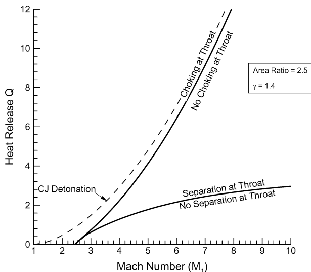
Fig. 10 Theoretically computed envelopes of operation for superdetonative ram accelerator.
