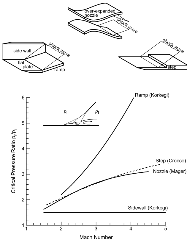
Fig. 7 Critical pressure ratio at which boundary-layer separation occurs as function of Mach number, as predicted by various theoretical and empirical correlations: Crocco 43 (flow separation in front of step), Mager 44 (free boundary separation), and Korkegi 45 (separation in front of wedge-supported shock).
