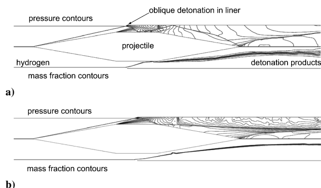
Fig. 15 Computational simulation of explosive line-ram accelerator showing pressure contours and mass fraction (hydrogen fill gas vs detonation products) at a) 12,000 m/s projectile velocity and b) 22,000 m/s projectile velocity.
