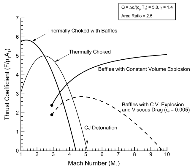
Fig. 13 Thrust on ram accelerator projectile (normalized by fill pressure and tube area) for possible modes of operation in baffled tube.
