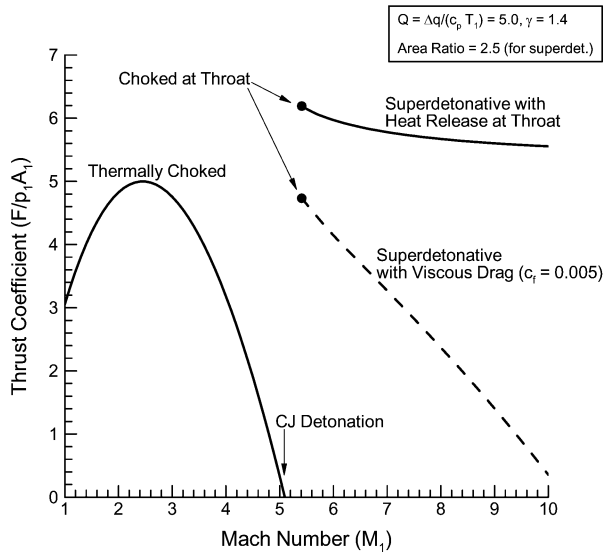
Fig. 2 Thrust on ram accelerator projectile (normalized by fill pressure and tube area) for thermally choked and superdetonative modes of operation.
