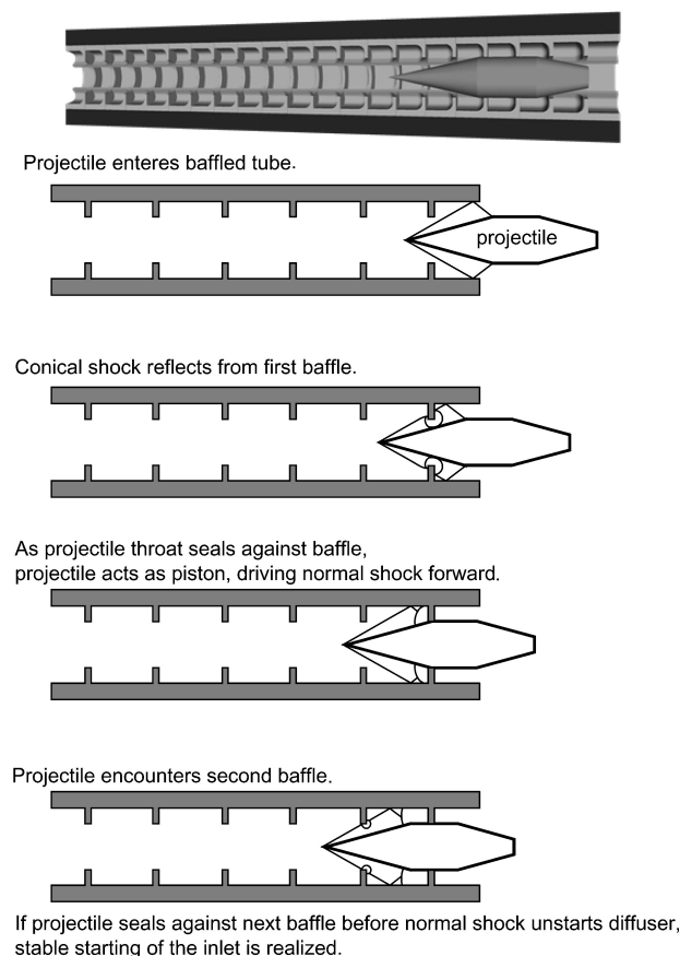
Fig. 12 Schematic of ram accelerator operation in baffled tube.
