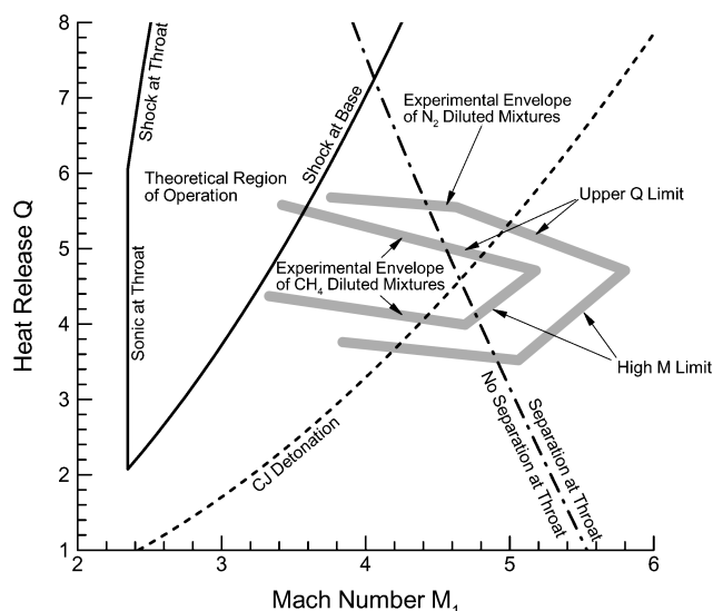
Fig. 4 Experimentally measured and theoretically computed envelopes of operation.
