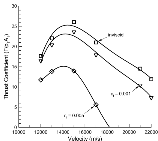
Fig. 16 Thrust on projectile in explosive-lined ram accelerator (normalized by hydrogen core fill pressure and tube area), as computed by surface pressure integration of computational simulation and using constant c_f skin-friction correction.
