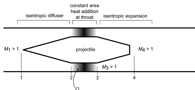
Fig. 9 Model of operation in superdetonative mode.
