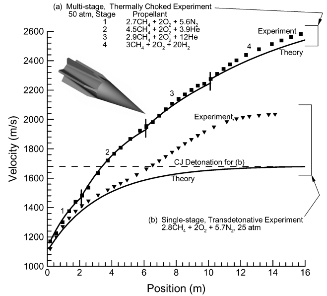
Fig. 3 Experimental velocity-position data from 38-mm University of Washington ram accelerator using 70-g projectile (shown) for a) multi-stage, thermally choked operation and b) single-stage, transdetonative operation.
