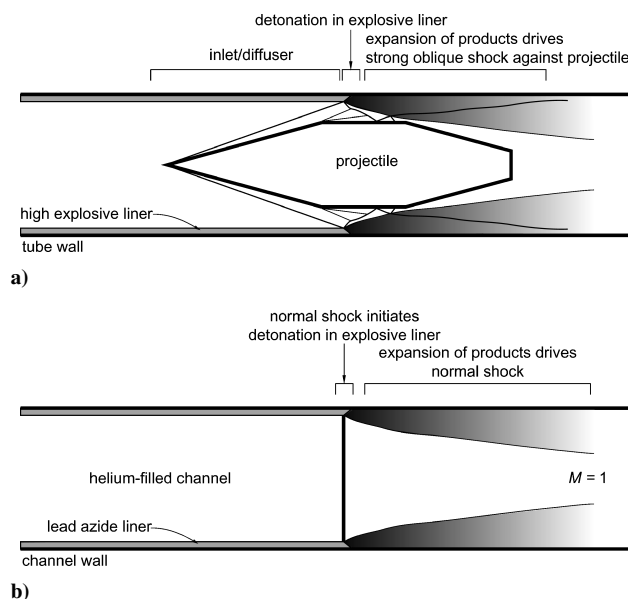
Fig. 14 Explosive-lined a) ram accelerator concept and b) channel experiment by Bakirov and Mitrofanov. 101
