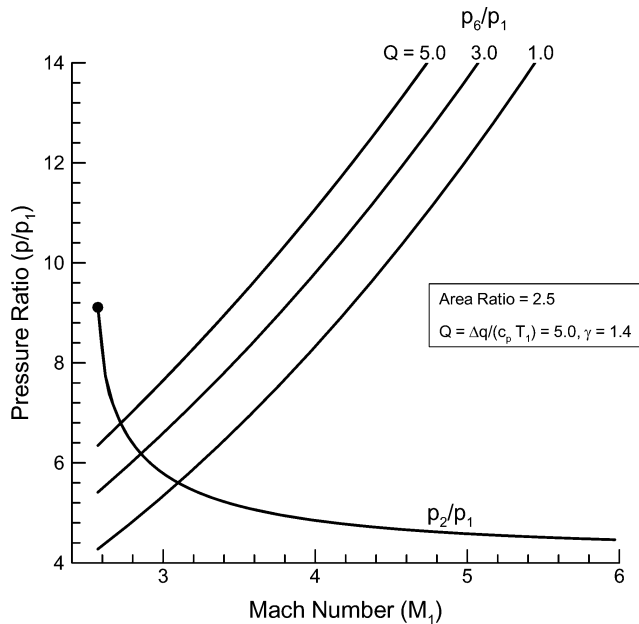
Fig. 6 Static pressure at projectile throat ( p_2 ) and sonic choking plane ( p_6 ) for different values of heat release as function of Mach number.
