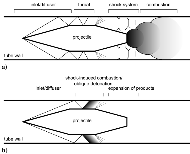
Fig. 1 Schematic of a) subdetonative, thermally choked ram accelerator flowfield and b) superdetonative ram accelerator.
