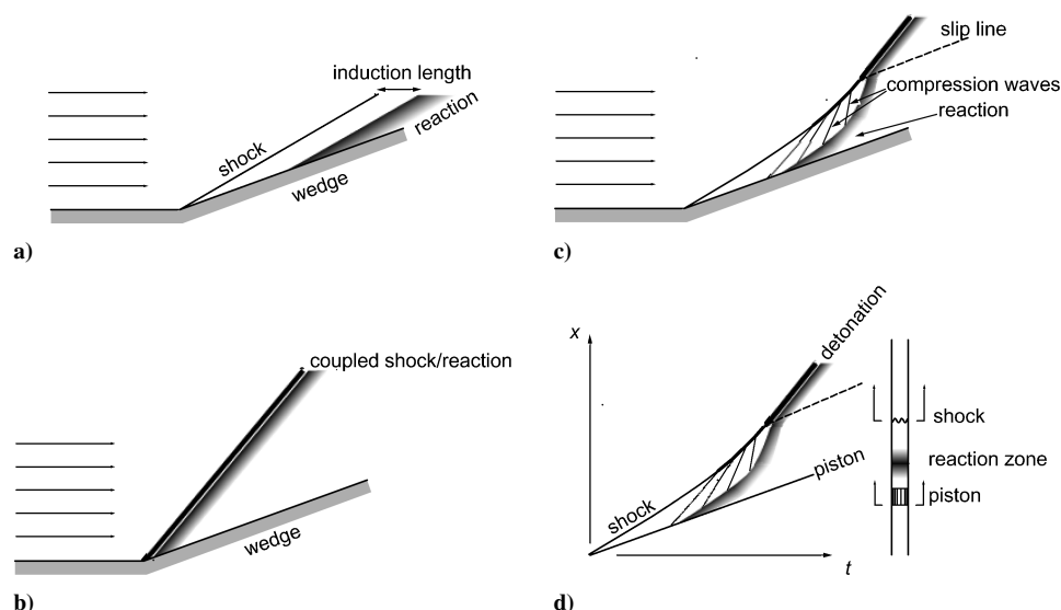
Fig. 8 Shock-induced supersonic combustion stabilized on wedge: a) shock-initiated combustion occurring at fixed distance downstream of oblique shock, b) oblique detonation with combustion coupled to shock, c) transition of shock-induced combustion to oblique detonation via compression waves generated by volumetric dilation of combustion products and d) analog to one-dimensional, piston-initiation detonation.
