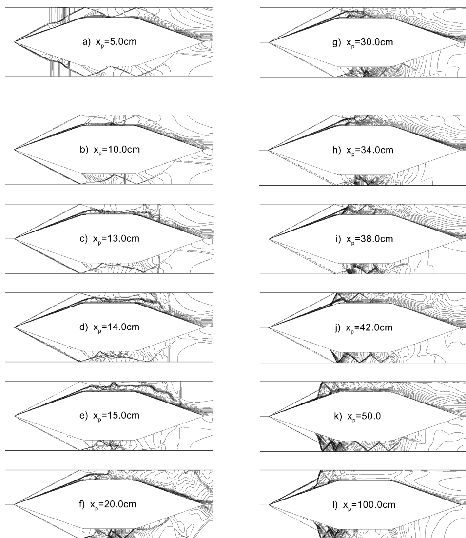
Fig. 11 Navier–Stokes simulation of superdetonative ram accelerator by Choi et al. 72 showing role of separation at projectile throat in unstart. Contours of temperature (upper-half) and pressure (lower-half) of flowfield are shown. Projectile injected at 2500 m/s into 2\text{H}_2 + \text{O}_2 + 5\text{N}_2 .
